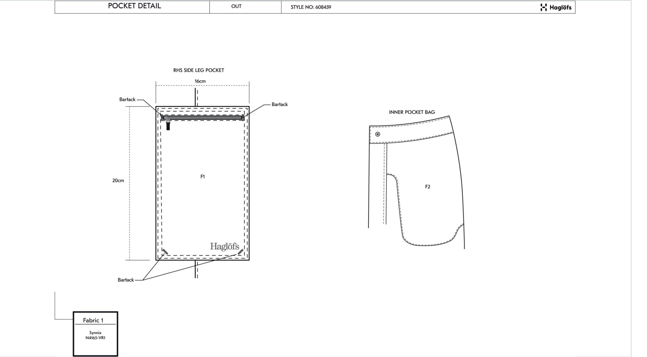
13. Detail Sketch 3
