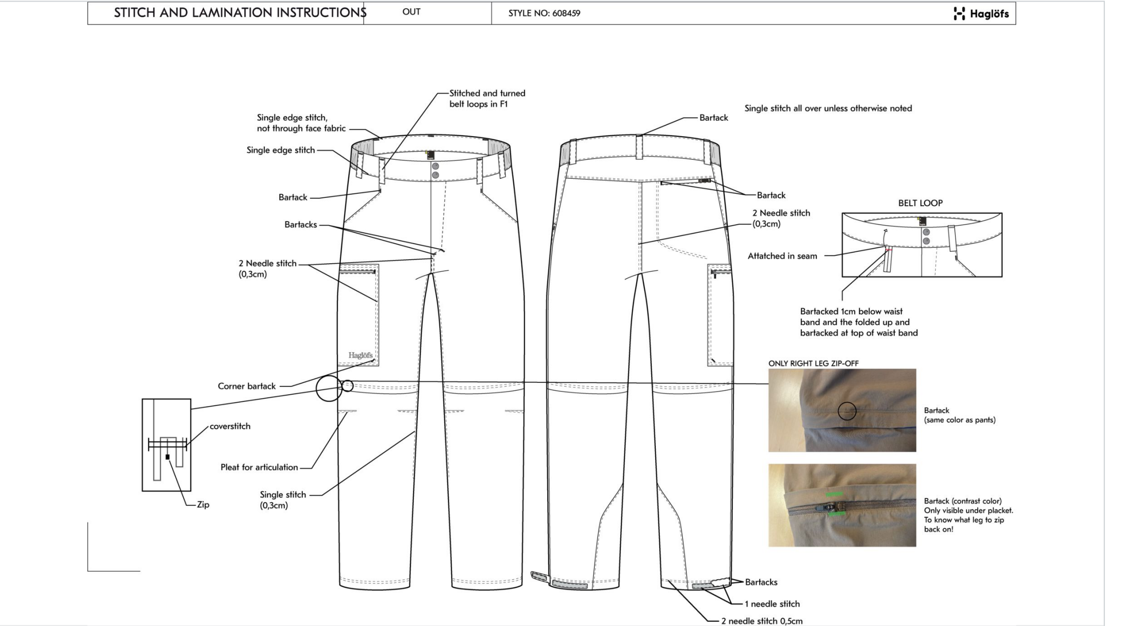
15. Detail Sketch 5
