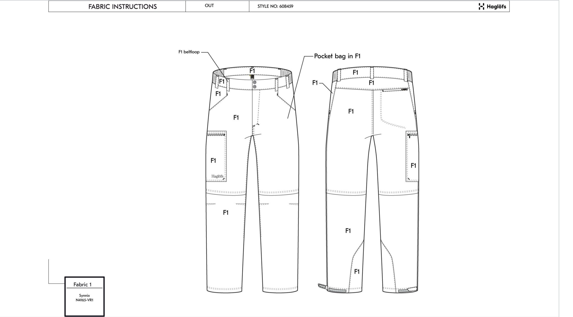
11. Detail Sketch 1
